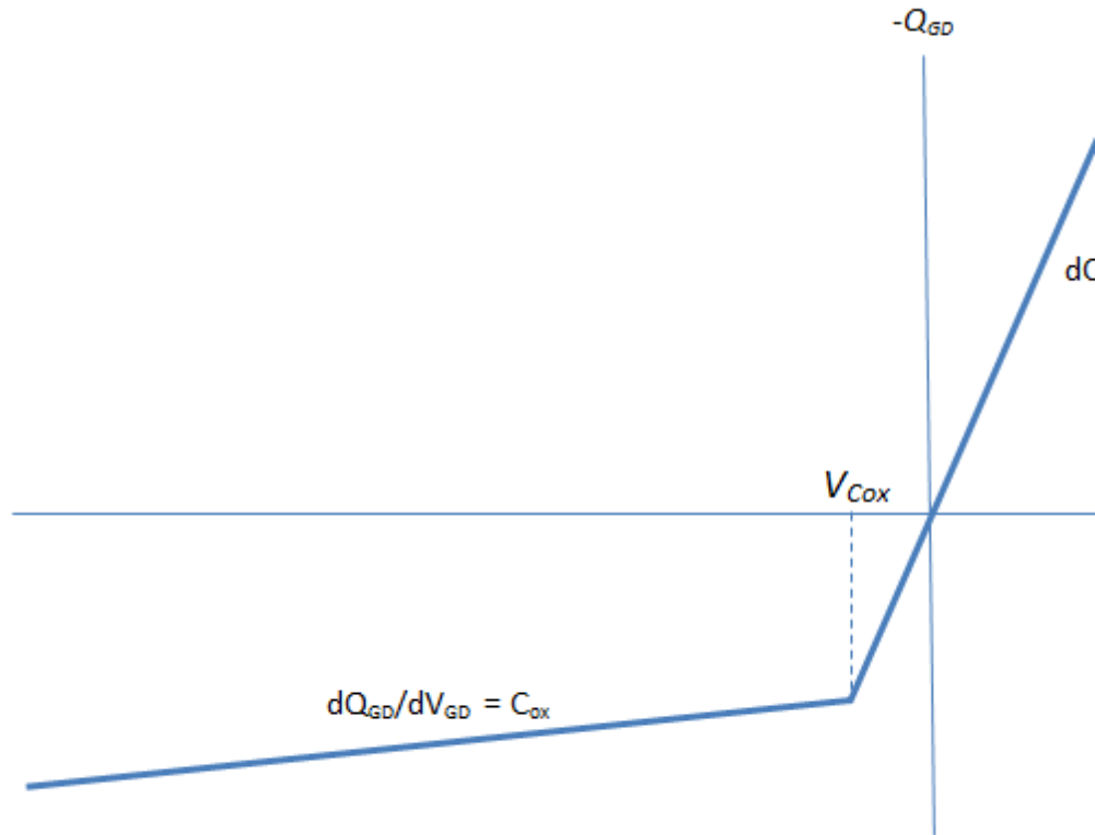
Nonlinear gate-drain charge function
