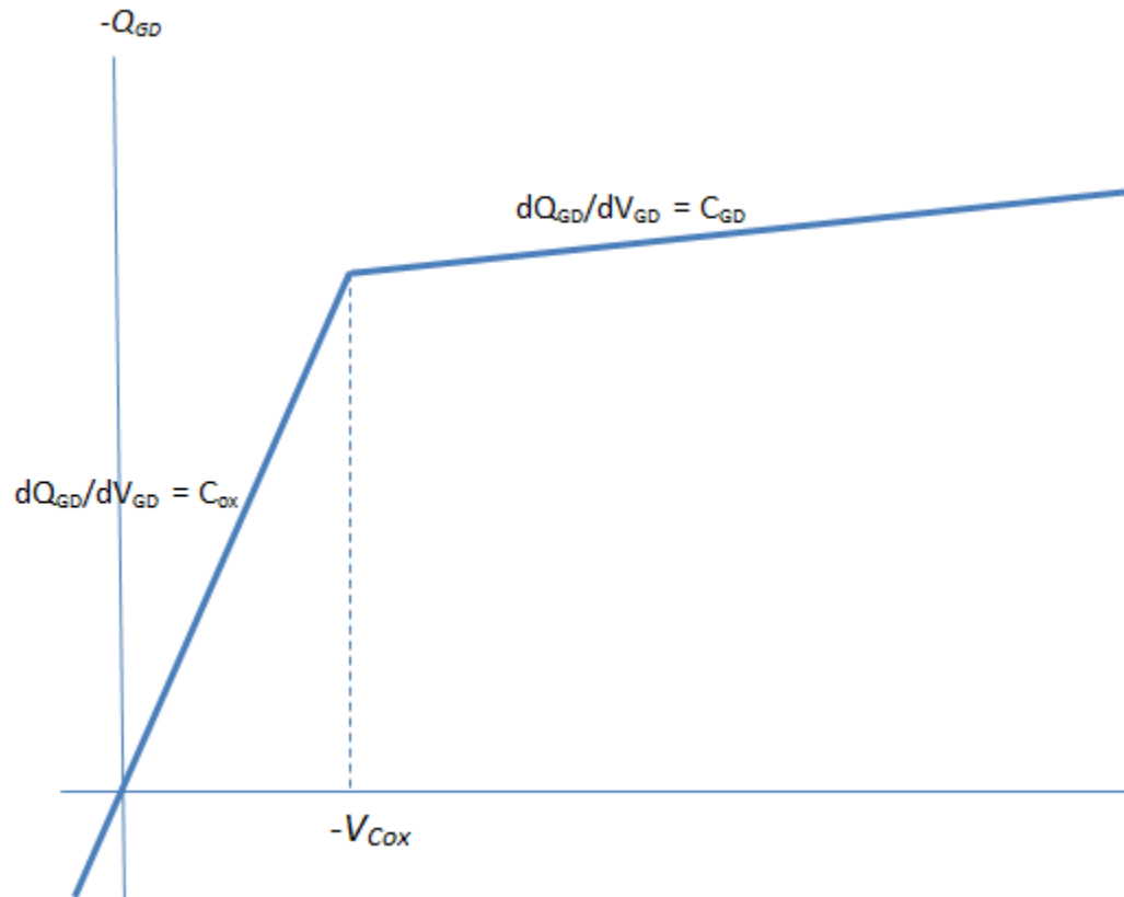
Nonlinear gate-drain charge function
